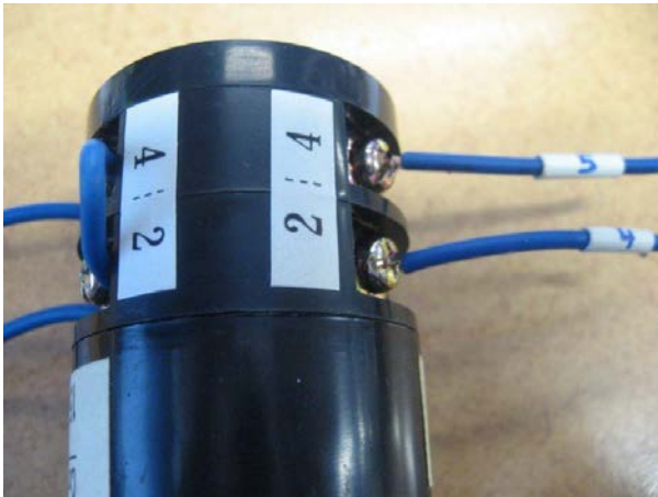
Wire 5 on pin 4 and wire 4 on pin 2 Note 4&2 are bridged
